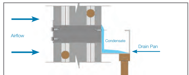
Intermediate drain pan for removal of condensate from coil banks.
